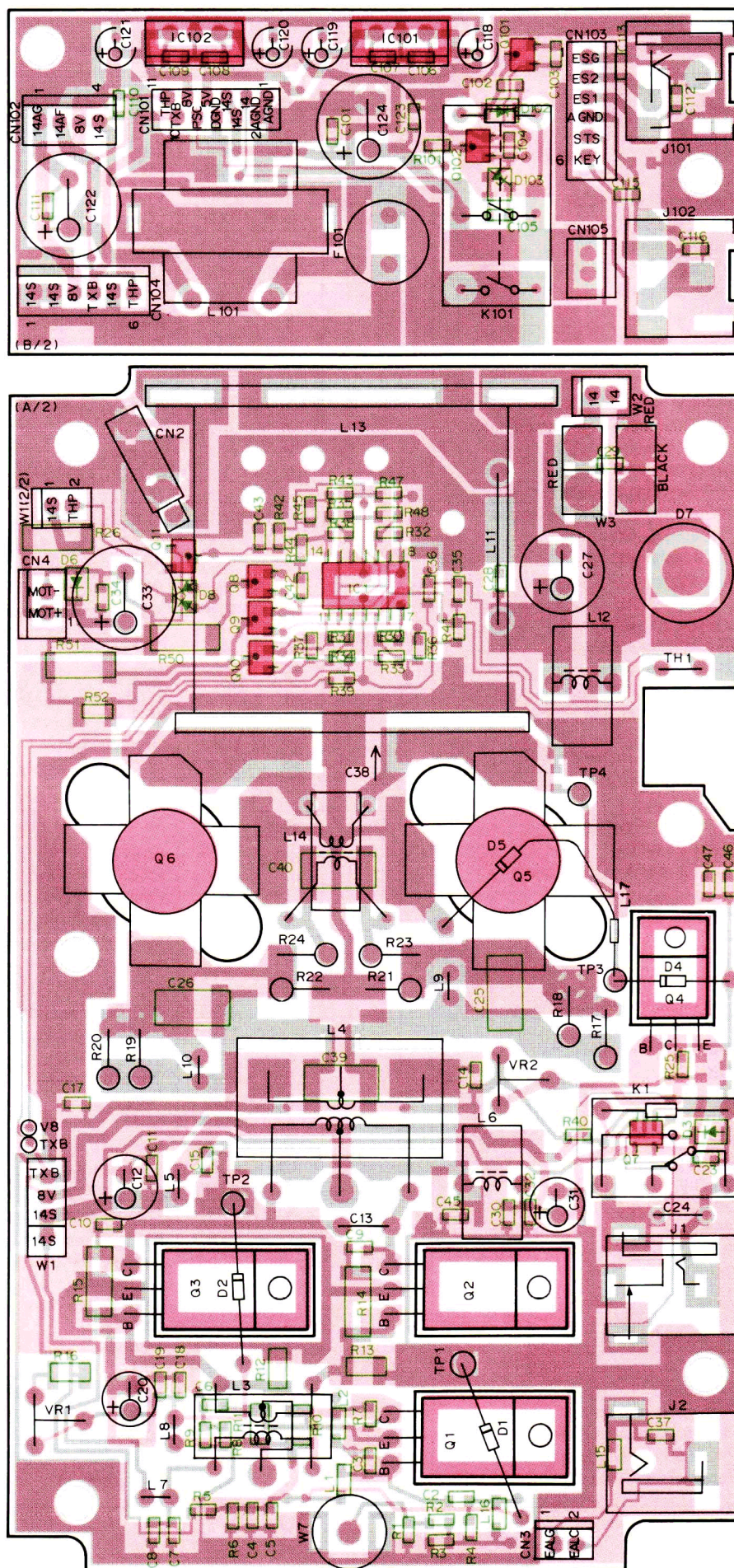
FINAL UNIT (X45-3460-00) Foil side view
