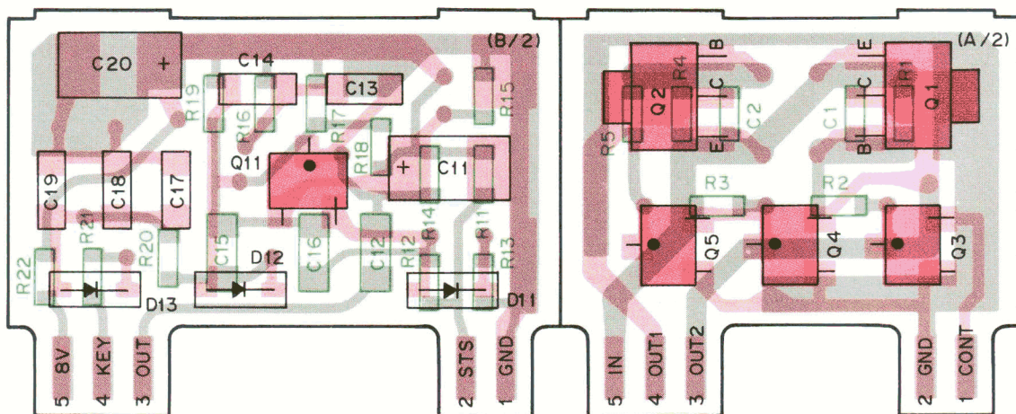
DSST (X59-4000-00) Foil side view
