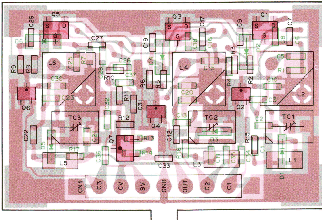
VCO (X58-4010-00) Foil side view
