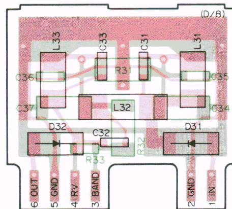
(D/8) Foil side view
