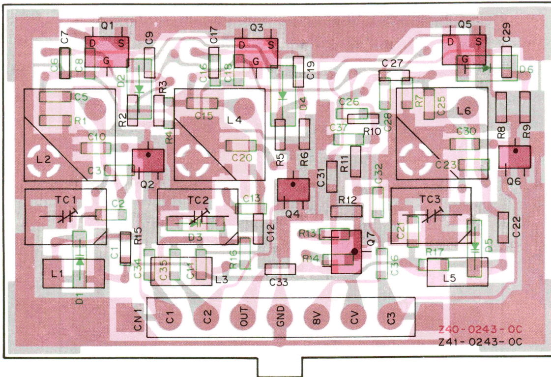
VCO (X58-4010-00) Component side view
